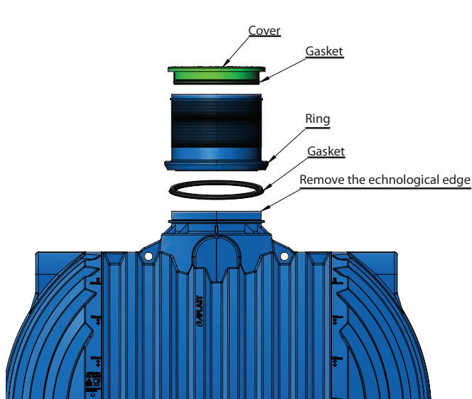
Figure 19: Ring installation option
