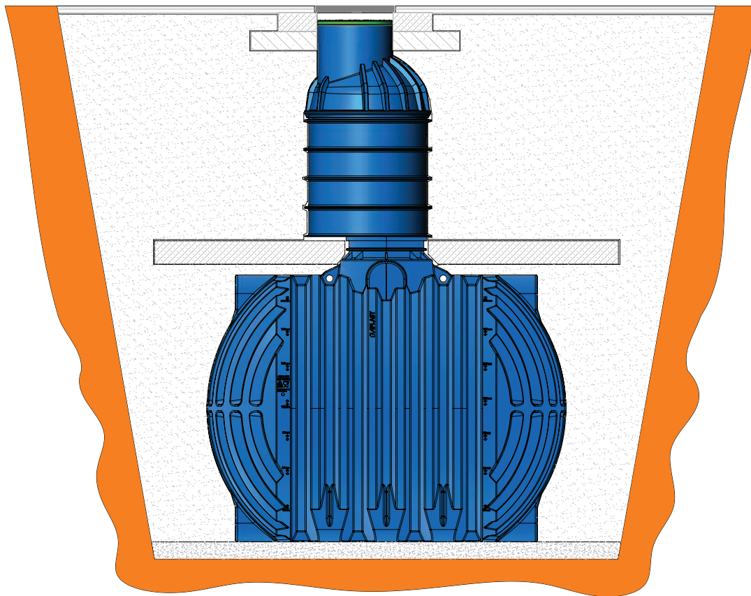
Figure 15: Installation of the tank in case of infilling over the allowed height
