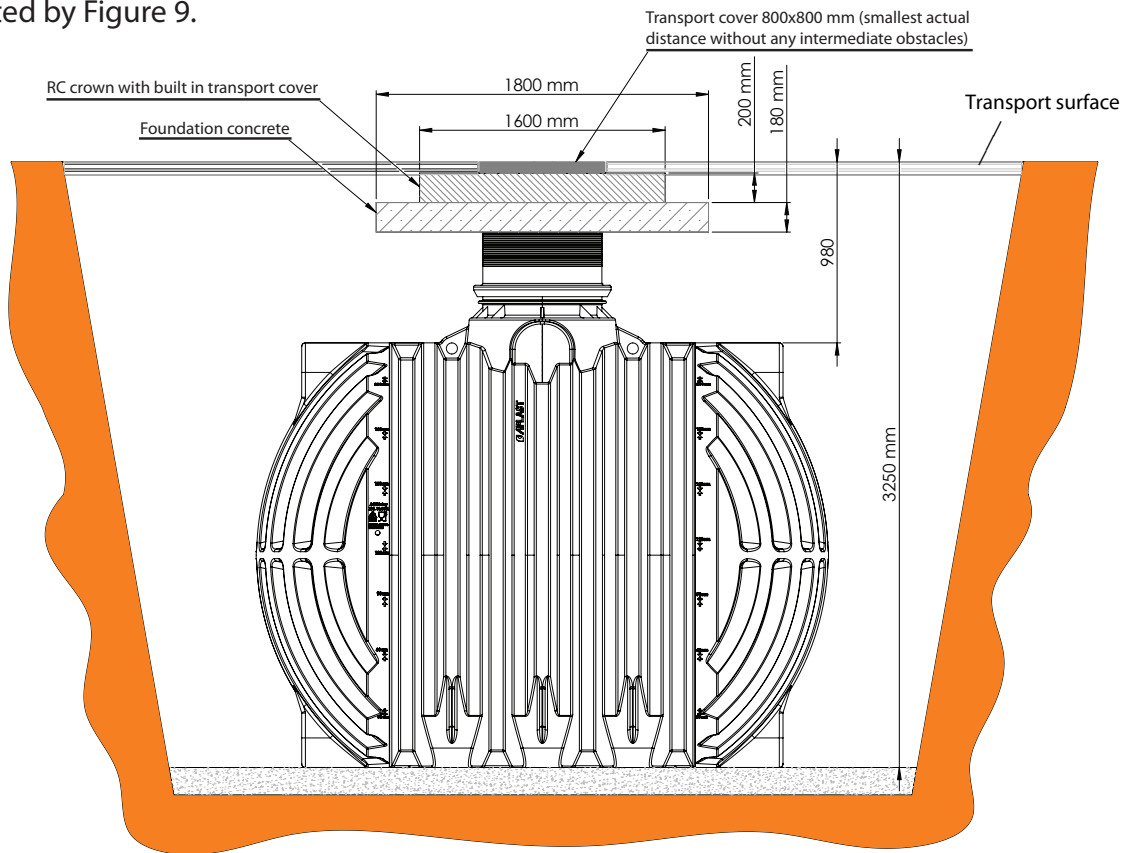
Figure 9: Installation of the tank under transport surfaces for vehicles with an axle load of up to 2.2 tonnes
