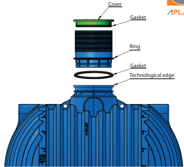
Figure 20: Extension ring installation option
