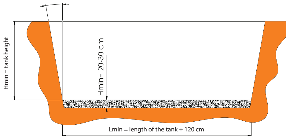
Figure 4: Construction pit
